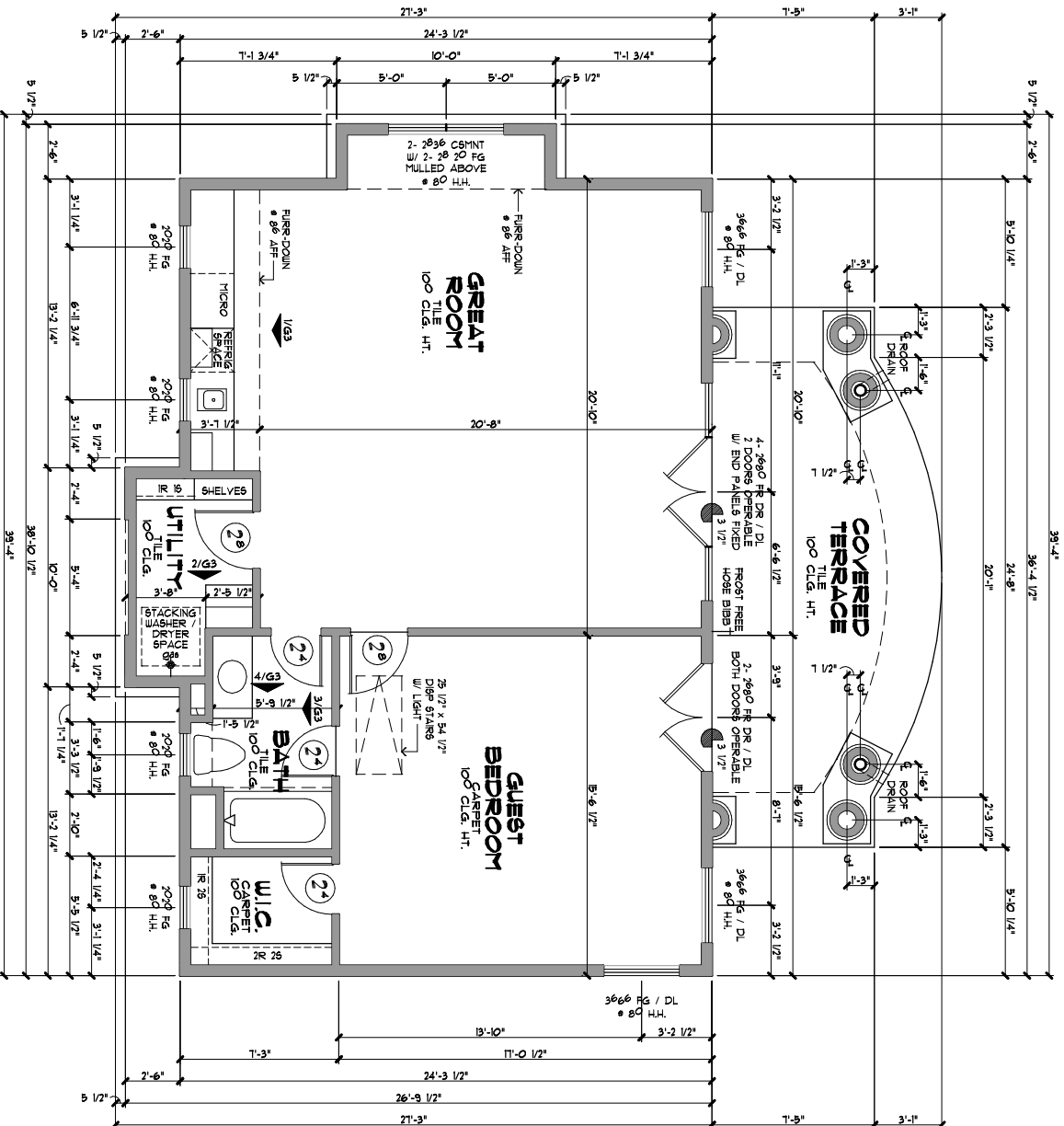
GUEST HOUSE FLOOR PLAN SCALE: 1/4" = 1'-0"
